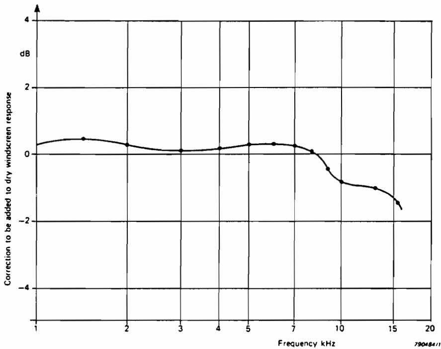
Fig.9.3. Effect of wet screen on the attenuation of Windscreen UA 0570
