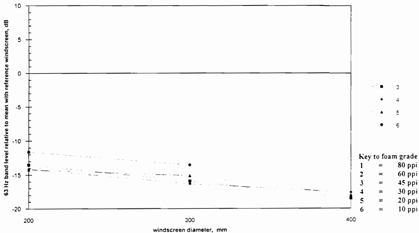
Figure 39 Two layer windscreens, 10 m/s. SPL in 63 Hz band -v- foam grade, different diameters
