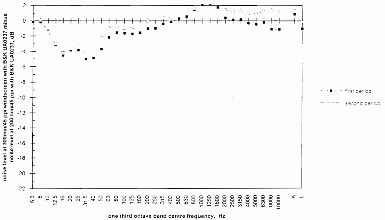
Figure 47 Comparative noise spectra. 200 mm/45 ppi -v- 300 mm/45 ppi windscreens
