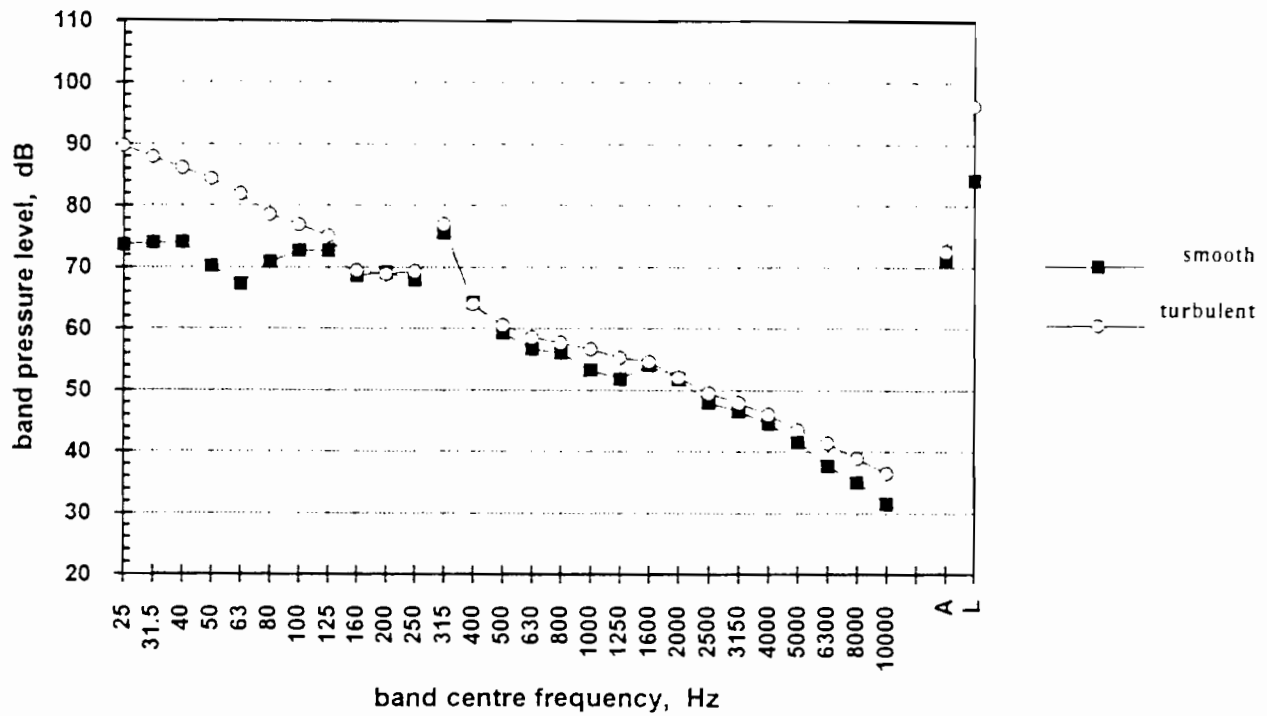
Figure 26 10 ppi solid windscreen -v-UA 0570 - smooth flow 10 m/s
