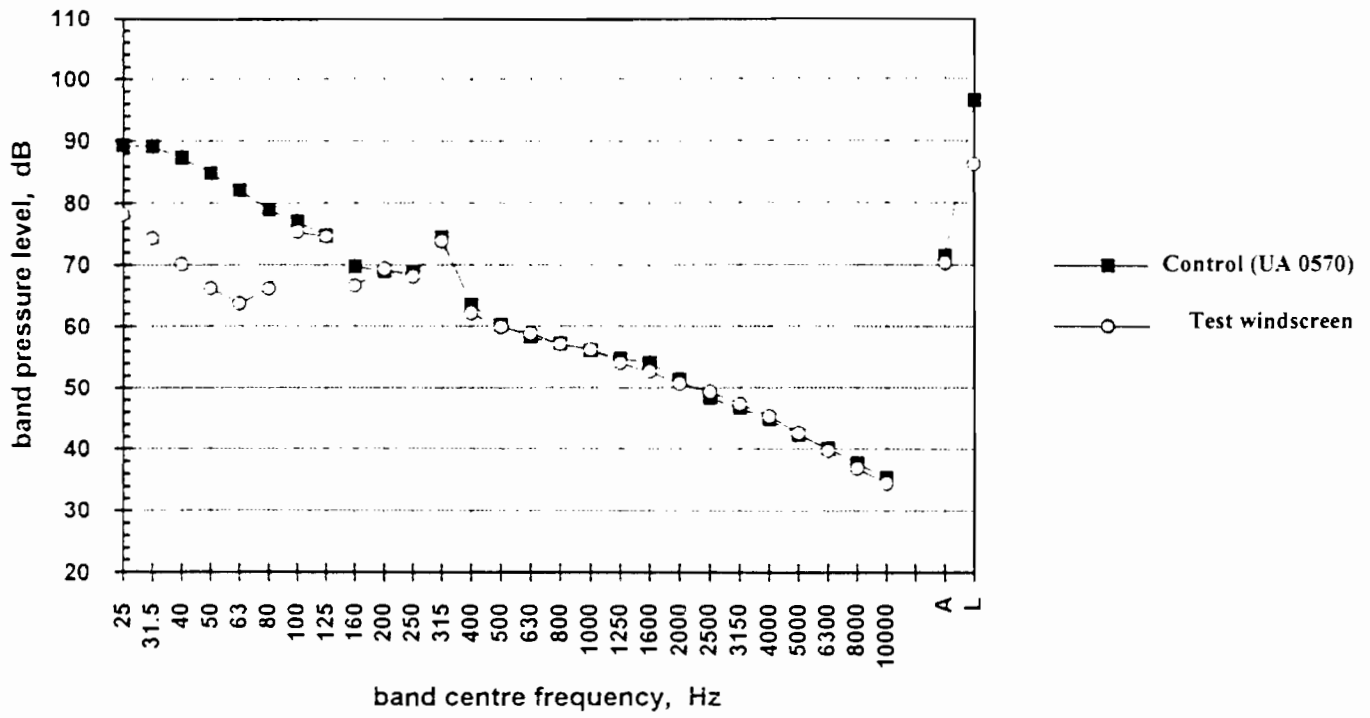
Figure 32 10 ppi solid windscreen -v- UA 0570 - turbulent flow 10 m/s
