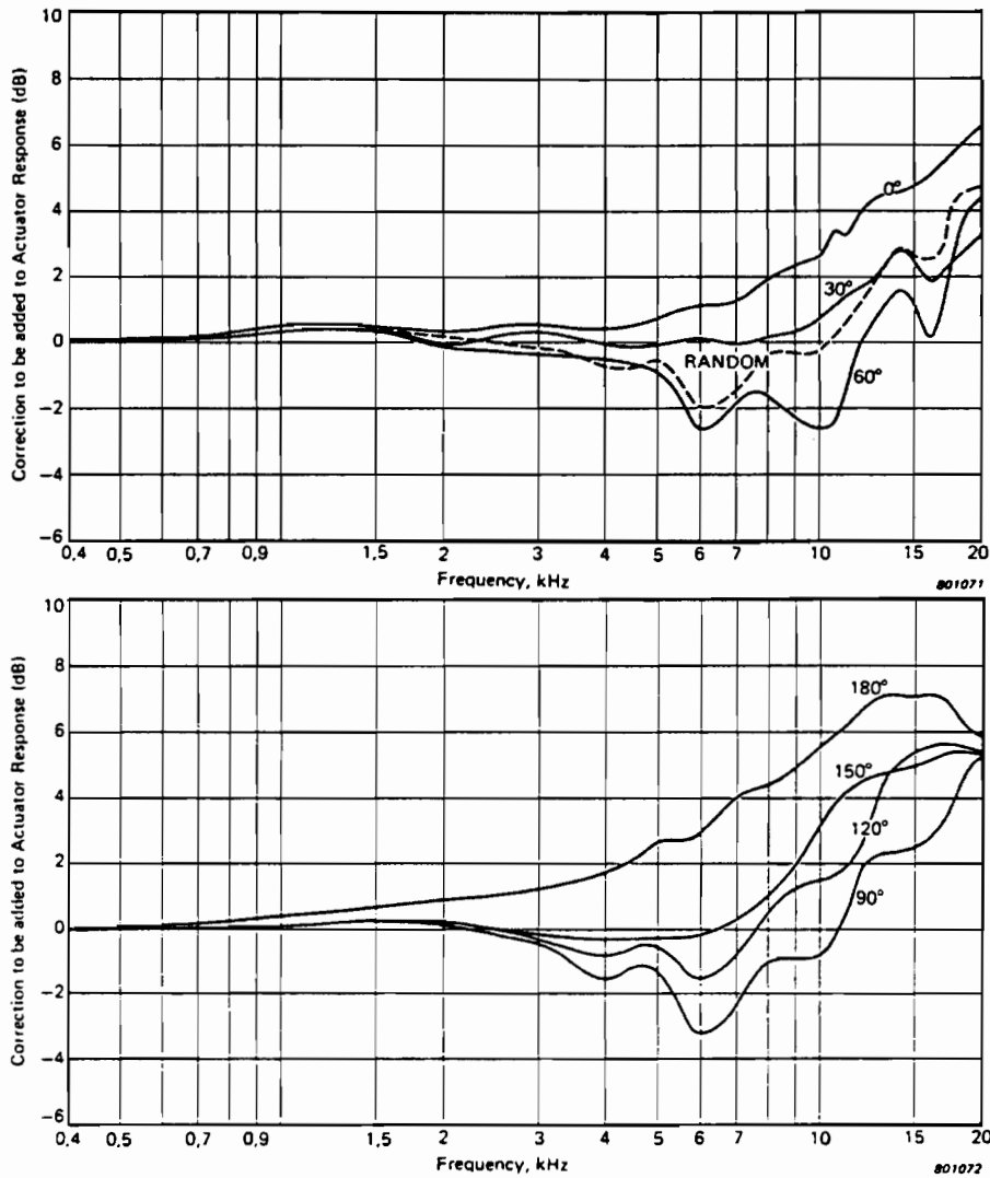
Fig. 9.7. Free-field correction curves for half-inch microphone Type 4133/49 fitted with Rain Cover UA 0393 and Dehumidifier UA 0308 mounted inside Windscreen UA 0570
