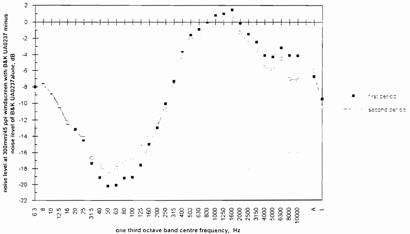
Figure 45 Comparative noise spectra. 300 mm/45 ppi -v- UA 0237 windscreens
