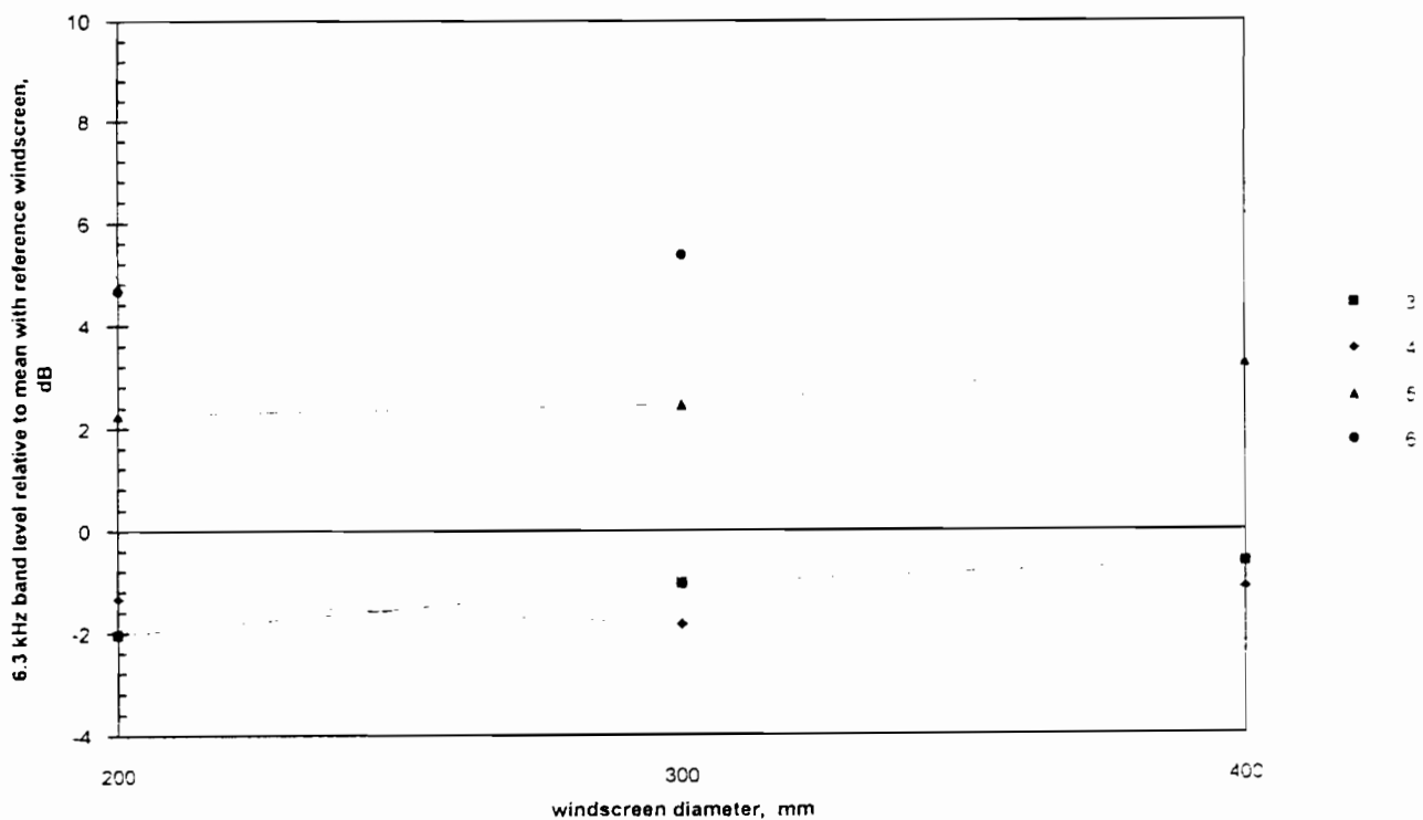
Figure 40 Two layer windscreens, 10 m/s. SPL in 6.3 kHz band -v- foam grade, different diameters
