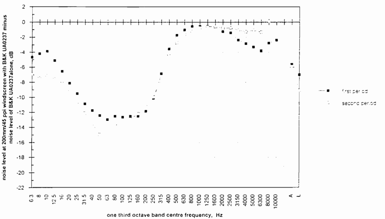
Figure 44 Comparative noise spectra. 200 mm/45 ppi -v- UA 0237 windscreens
