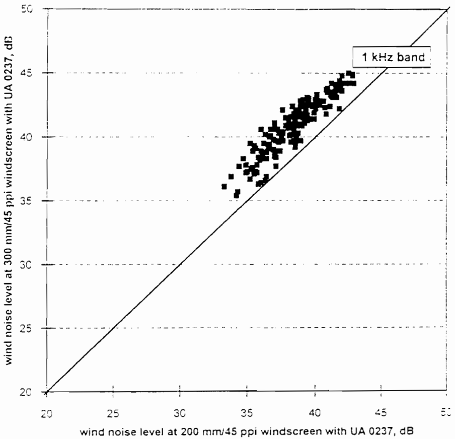
Figure 52 SPL in 63 Hz and 1 kHz bands plotted for 300 mm/45 ppi and 200 mm/45 ppi windscreens
