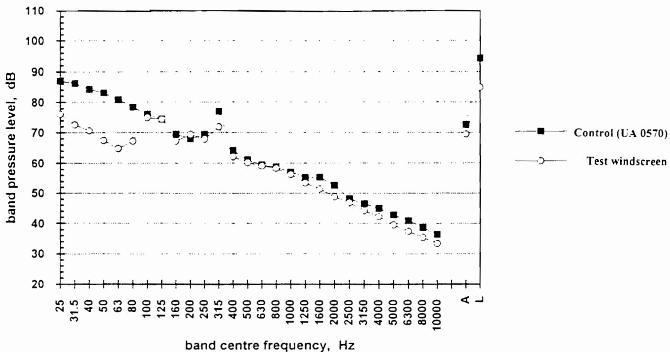
Figure 28 30 ppi hollow windscreen -v- UA 0570 - turbulent flow 10 m/s
