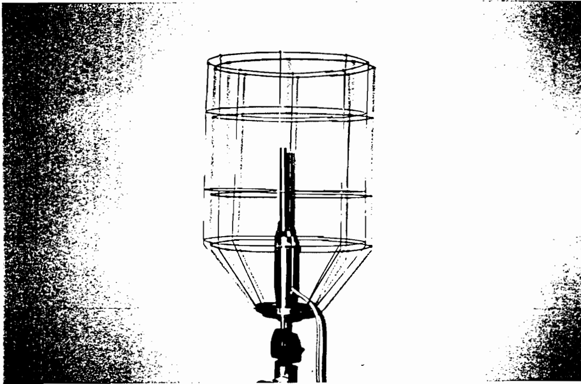
Figure 3 Frame construction for test windscreens, showing microphone and pre-amplifier mounted
