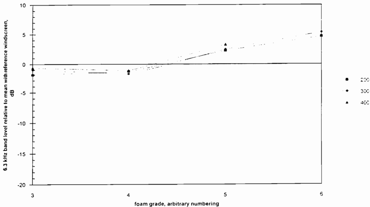
Figure 42 Two layer windscreens, 10 m/s. SPL in 6.3 kHz band -v- foam grade, different diameters
