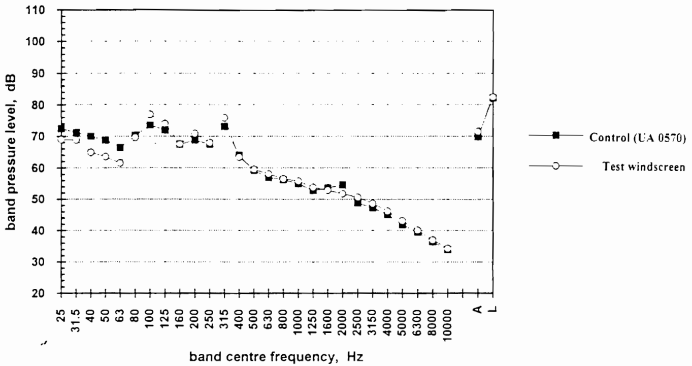
Figure 26 10 ppi solid windscreen -v-UA 0570 - smooth flow 10 m/s
