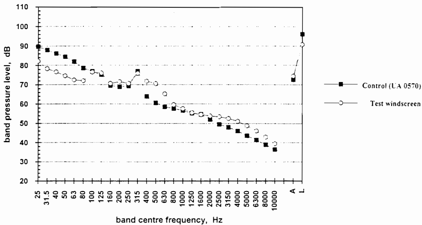
Figure 30 10 ppi hollow windscreen -v- UA 0570 - turbulent flow 10 m/s
