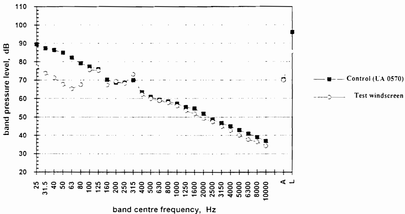
Figure 29 30 ppi hollow windscreen + UA 0237 -v- UA 0570 - turbulent flow
