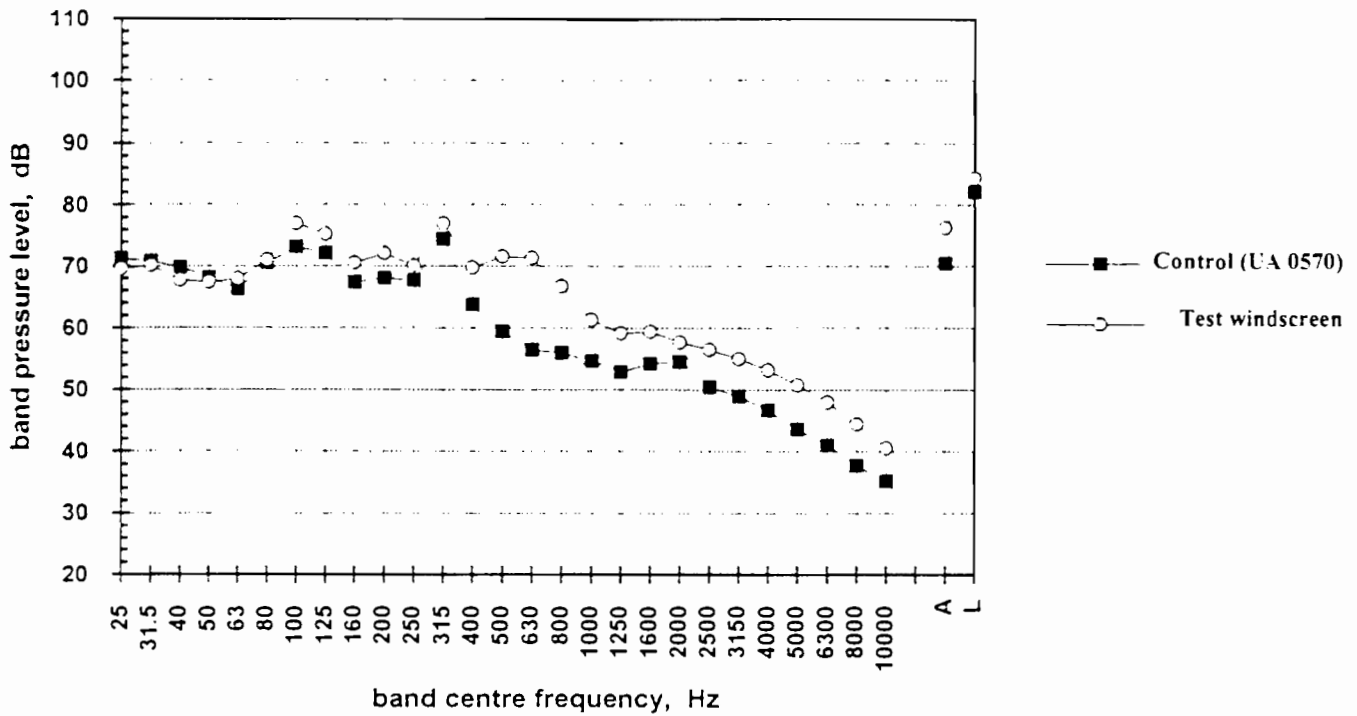
Figure 24 10 ppi hollow windscreen -v- UA 0570 - smooth flow 10 m/s
