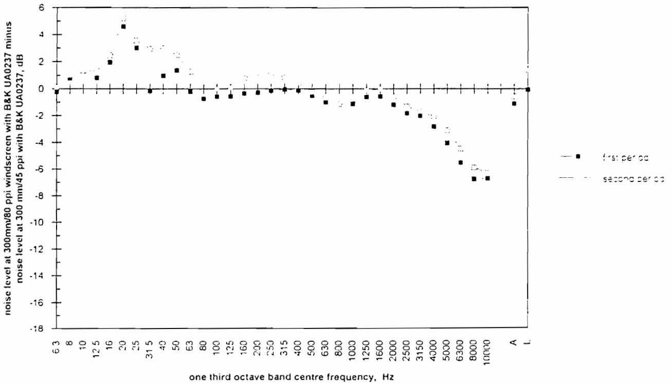
Figure 49 Comparative noise spectra. 300 mm/45 ppi -v- 300 mm/80 ppi windscreens
