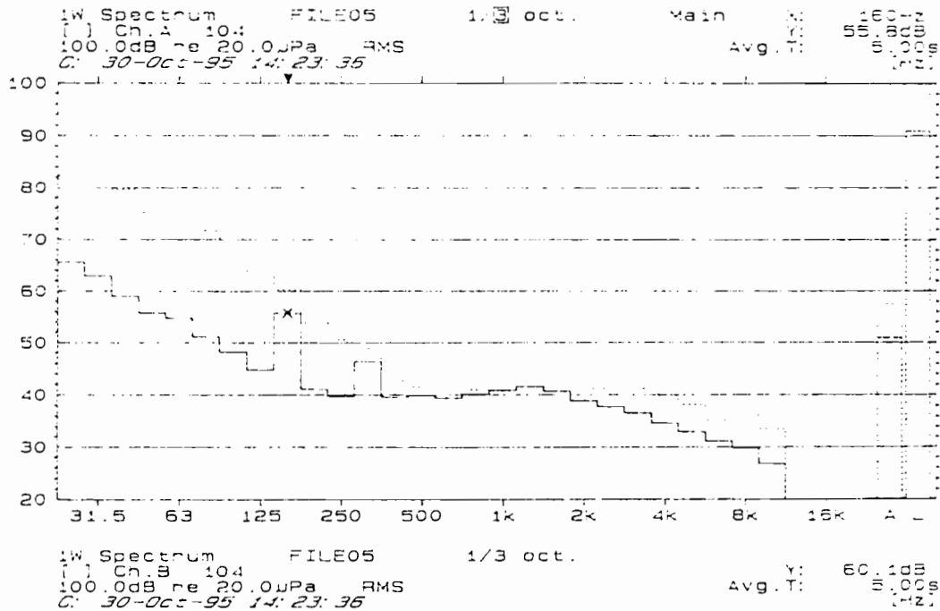
Figure 53 Typical frequency spectra ( L_{eq,5s} ) measured in wind. Upper spectrum - UA 0237 windscreen. Lower spectrum - 300 mm/45 ppi windscreen
