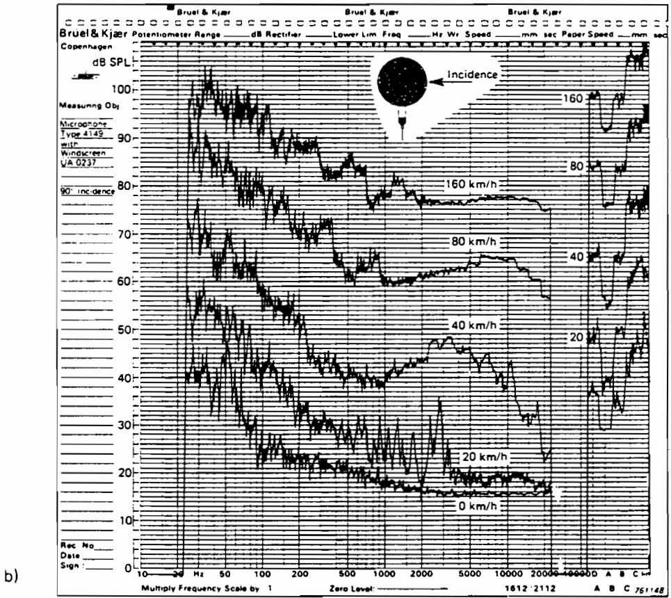
Fig.9.10. Wind induced noise levels for half-inch microphones fitted with Windscreen UA 0237 a) 0° incidence b) 90° incidence
