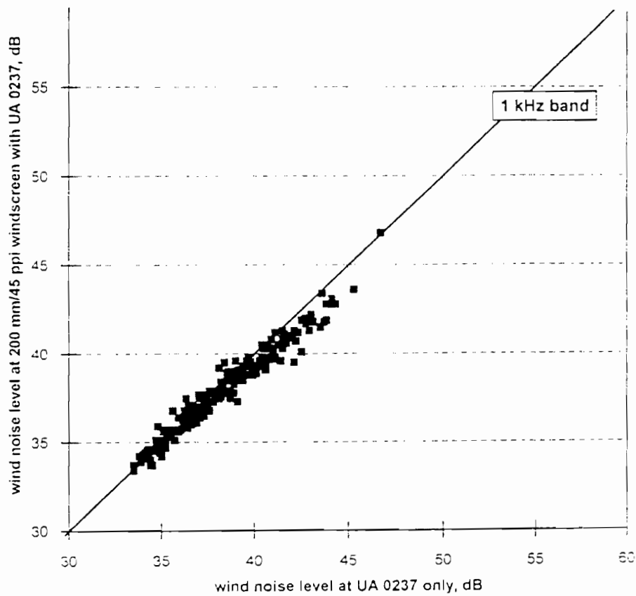
Figure 50 SPL in 63 Hz and 1 kHz bands plotted for 200 mm/45 ppi and UA 0237 windscreens
