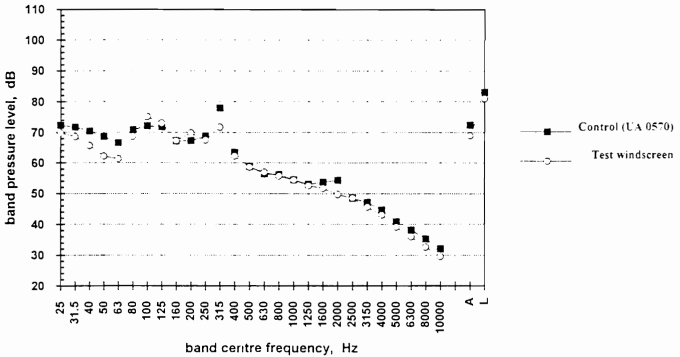
Figure 23 30 ppi hollow windscreen + UA 0237 -v- UA 0570 - smooth flow 10 m/s
