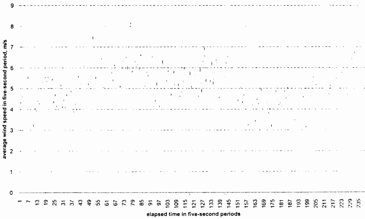
Figure 56 Typical time history of 5-second averaged wind speed over a 20 minute period at Farley Mount
