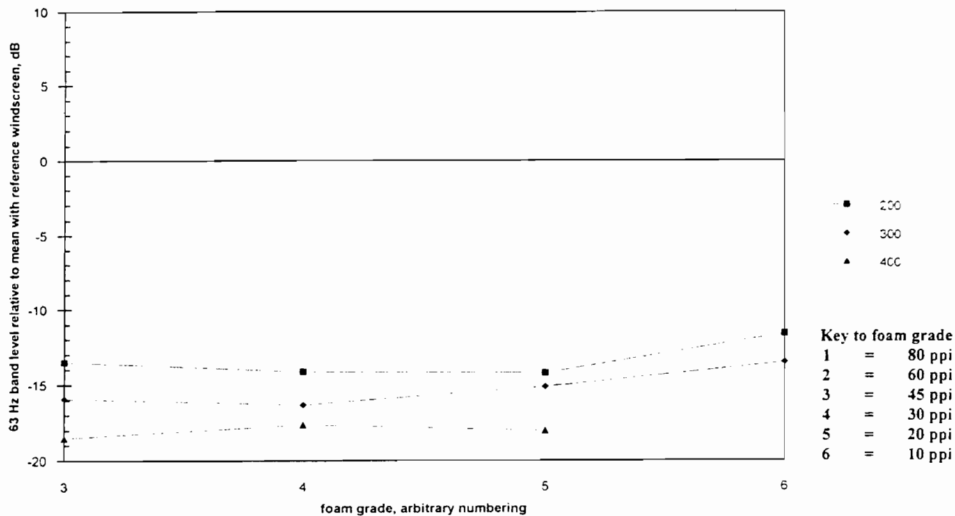
Figure 41 Two layer windscreens, 10 m/s. SPL in 63 Hz band -v- foam grade, different diameters
