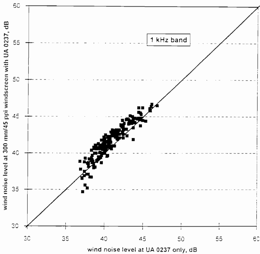
Figure 51 SPL in 63 Hz and 1 kHz bands plotted for 300 mm/45 ppi and UA 0237 windscreens
