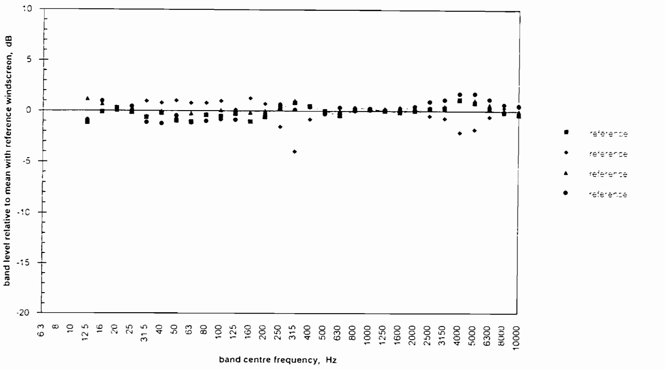
Figure 35 One-third octave band SPL/s relative to control windscreen (10 m/s) Two layer windscreens. 300 mm/45-30-20-10 ppi
