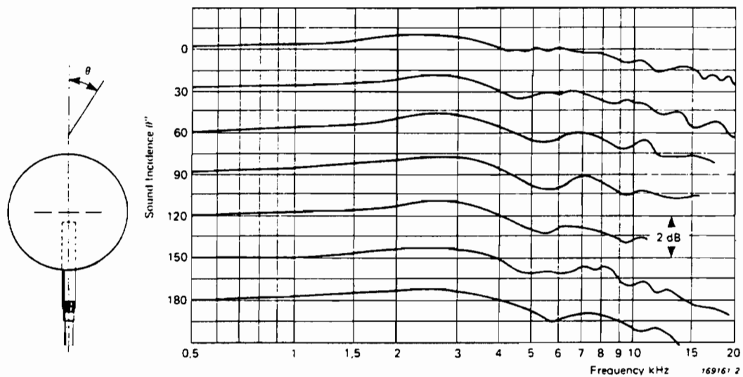
Fig.9.12. Increments to free-field correction curves due to Wind-screen UA 0237
