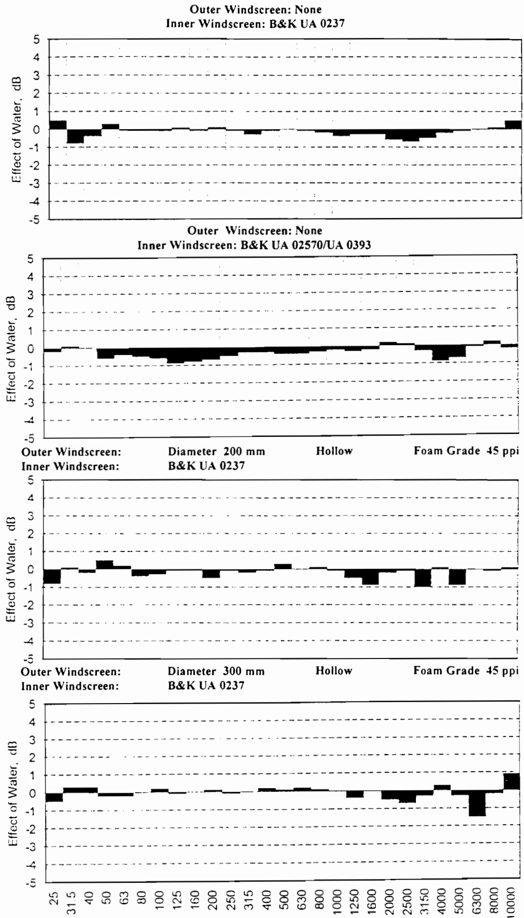
Figure 55 Effect of water absorption on acoustic insertion loss of windscreens
