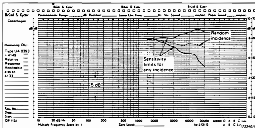
Fig.9.15. Sensitivity limits for any incidence for half-inch microphones Types 4133 and 4149 fitted Rain Cover UA 0393
