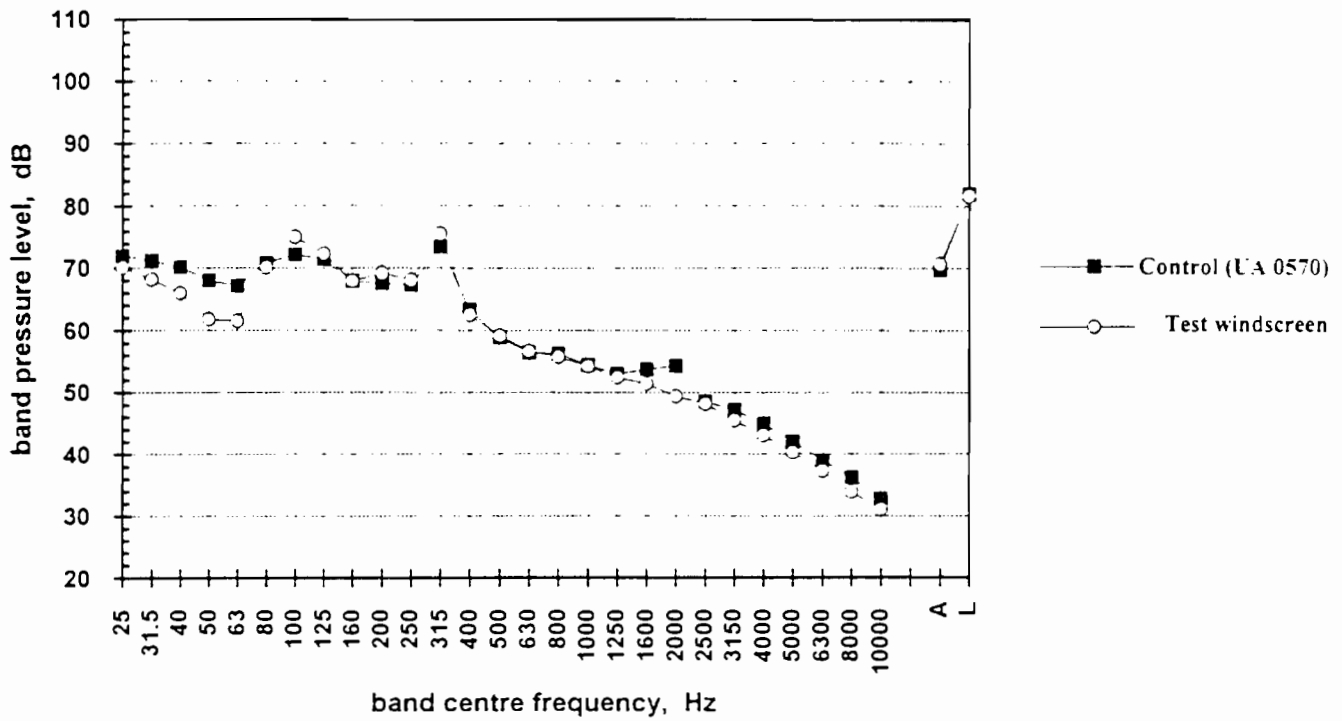
Figure 22 30 ppi hollow windscreen -v- UA 0570 - smooth flow 10 m/s
