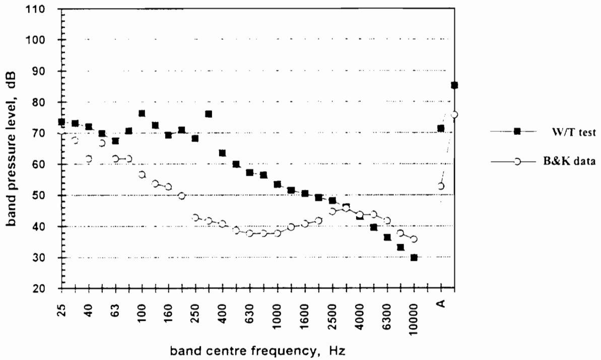
Figure 20 UA 0237 in wind tunnel -v- B&K data for wind noise (10 m/s)
