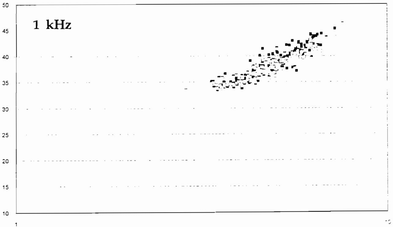
Figure 58 Scatter diagram - 5 second averaged SPL in 63 Hz and 1 kHz bands -v- wind speed m/s
