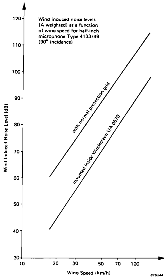
Fig. 9.5. A-weighted wind induced noise level as a function of wind speed for half-inch microphone Type 4133/49 fitted with Rain Cover UA 0393 and Dehumidifier UA 0308 mounted inside Windscreen UA 0570
