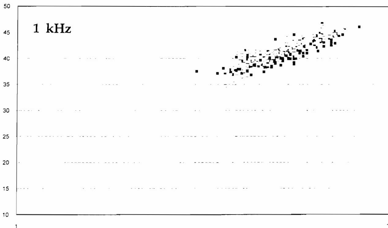
Figure 57 Scatter diagram - 5 second averaged SPL in 63 Hz and 1 kHz bands -v- wind speed m/s
