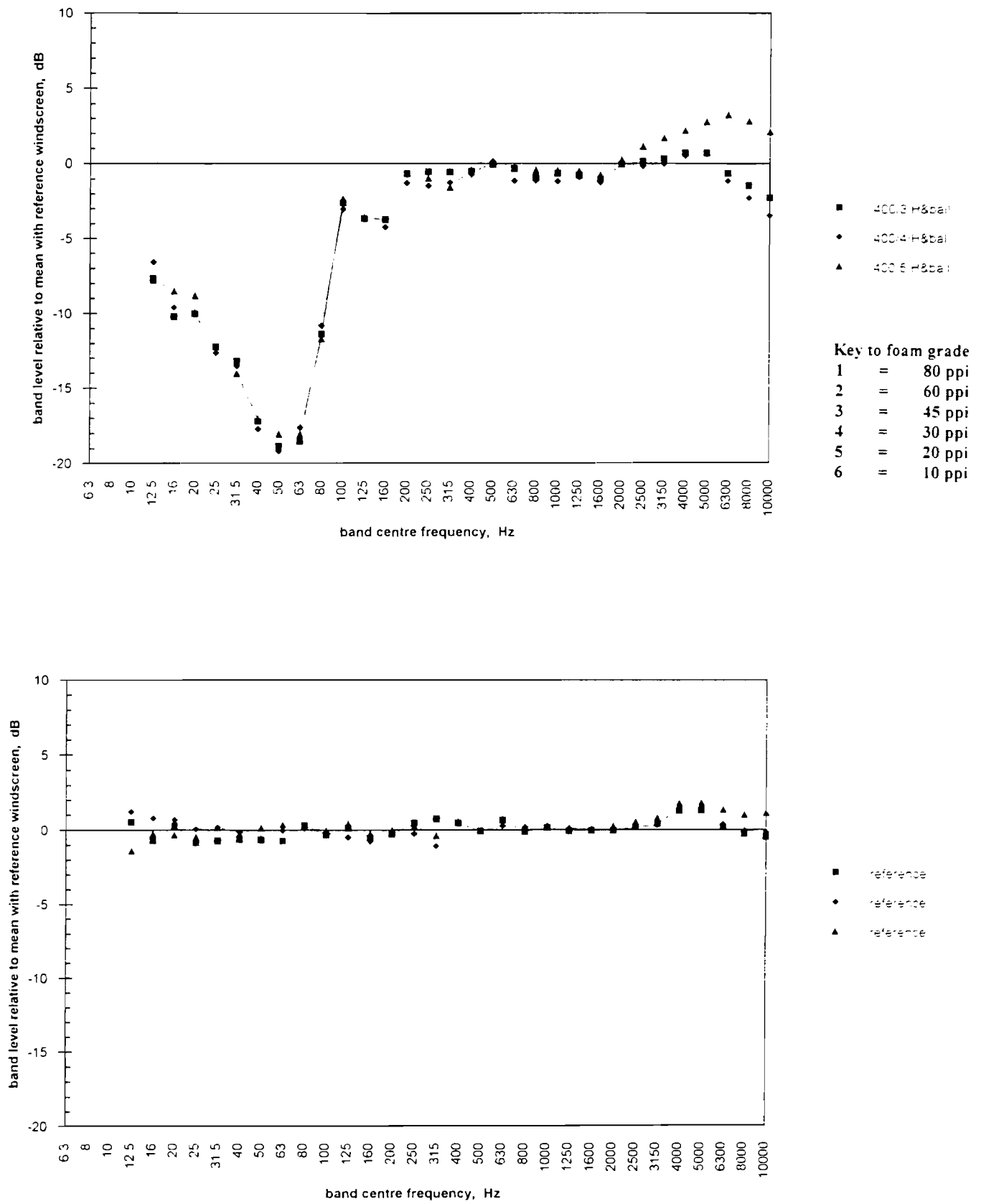
Figure 36 One-third octave band SPL/s relative to control windscreen (10 m/s) Two layer windscreens. 400 mm/45-30-20 ppi
