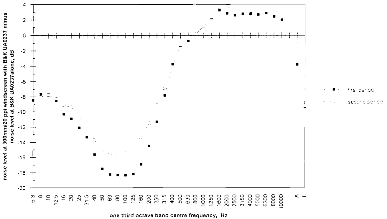
Figure 46 Comparative noise spectra. 300 mm/20 ppi -v- UA 0237 windscreens
