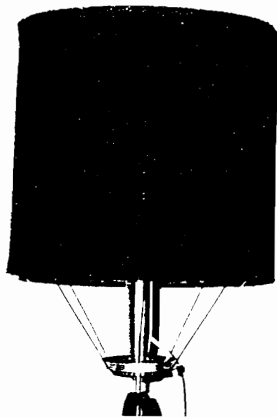
Figure 4 Installation of outer sleeve (10 ppi) on windscreen
