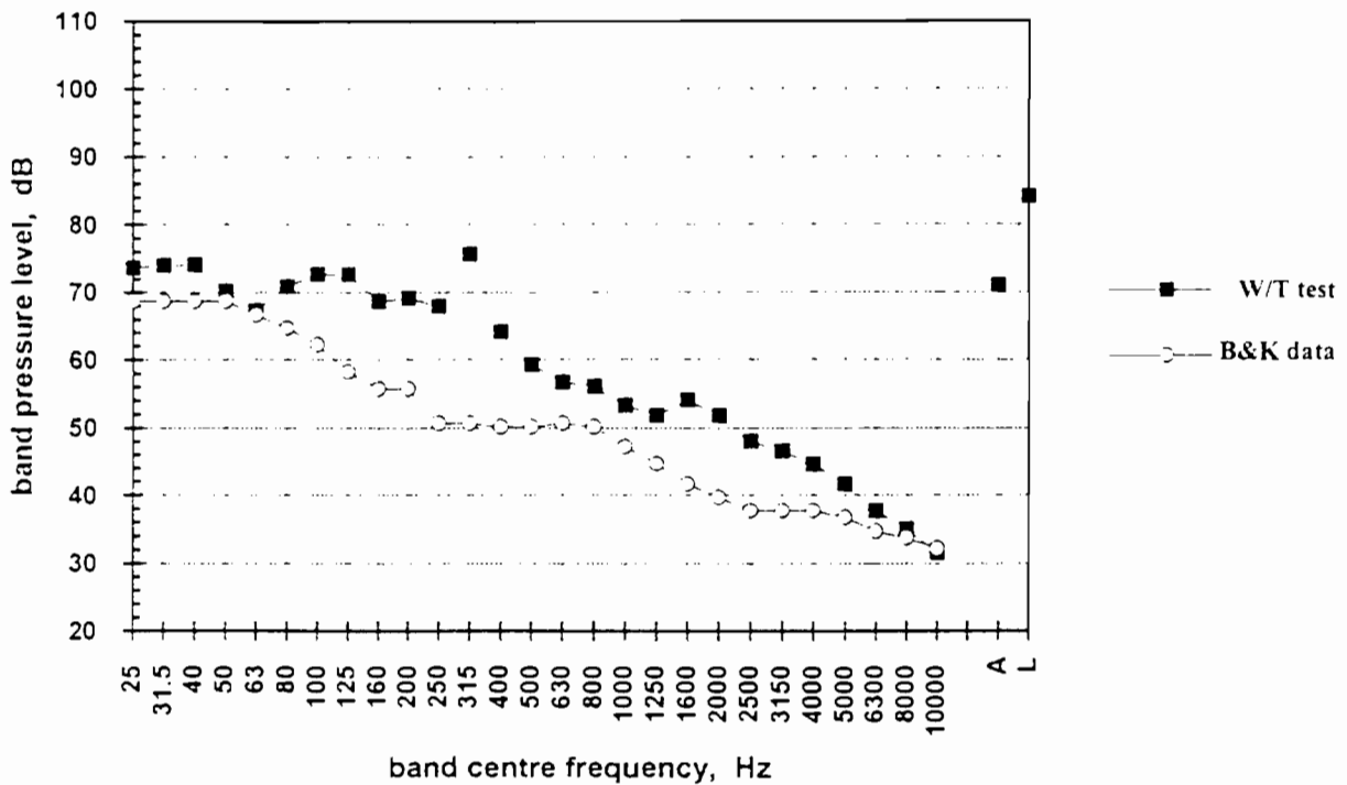
Figure 21 UA 0570 in wind tunnel (without 0393) -v- B&K data for wind noise
