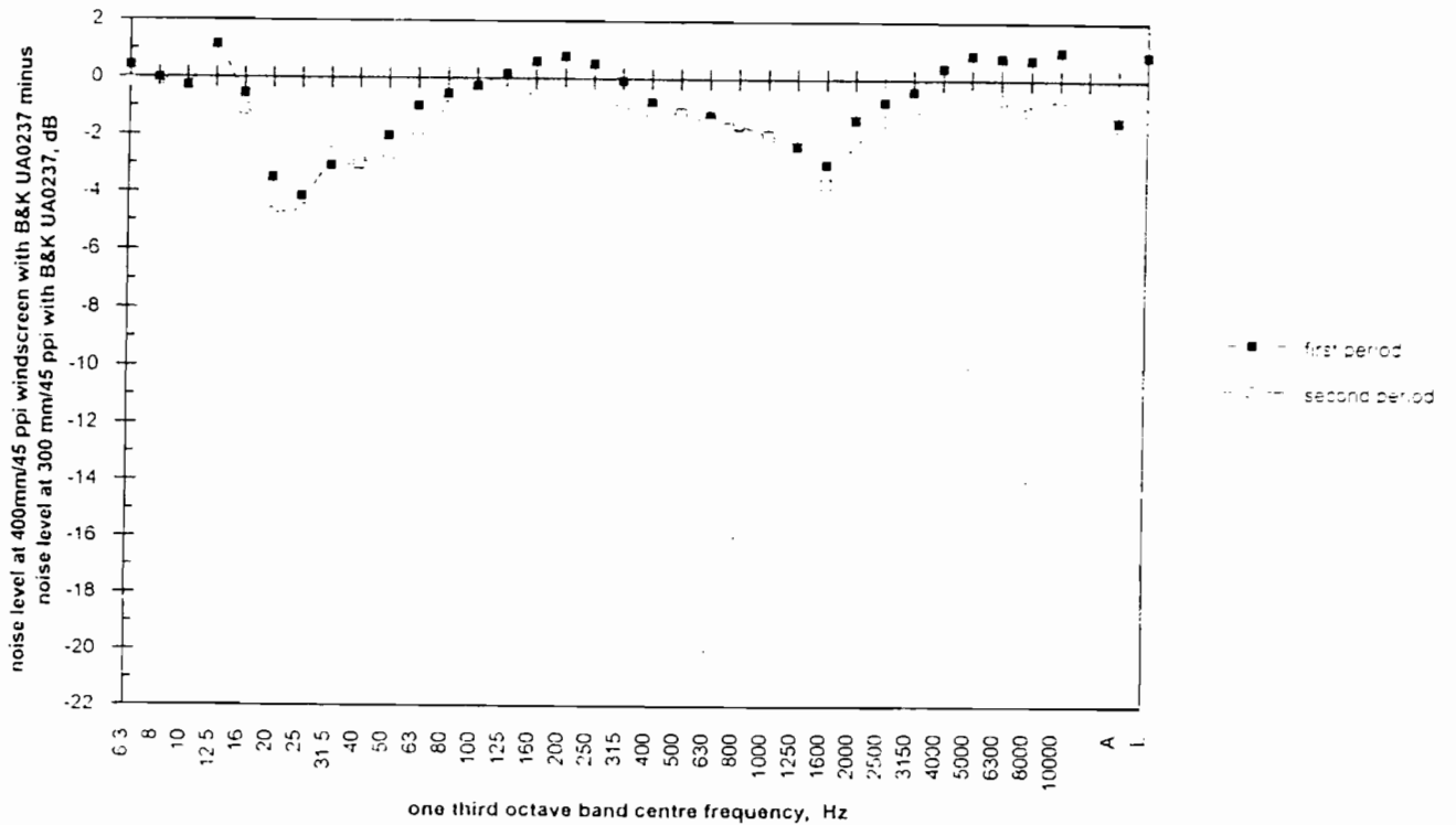
Figure 48 Comparative noise spectra. 300 mm/45 ppi -v- 400 mm/45 ppi windscreens
